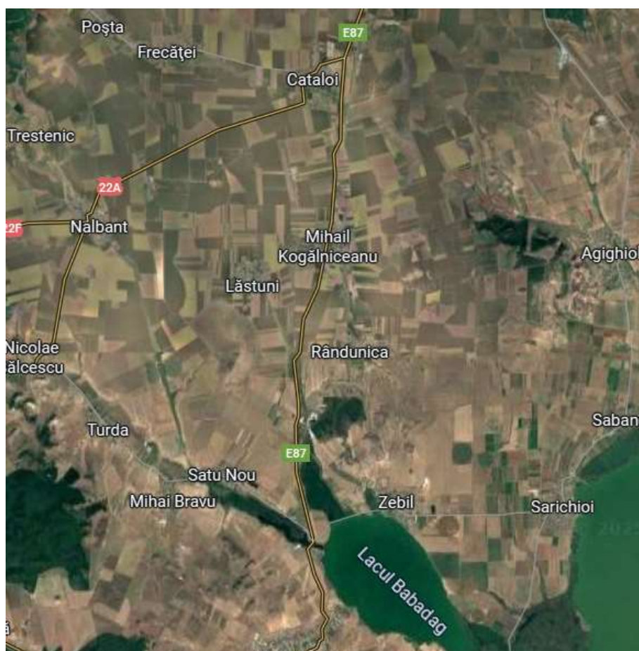
Figura 1 – Traseul DN22 = km 186+900 – km 210+000
